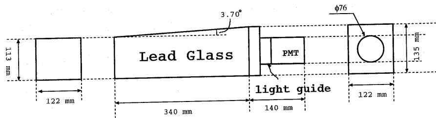
Figure 2.33: One cell of LG Calorimeter.
