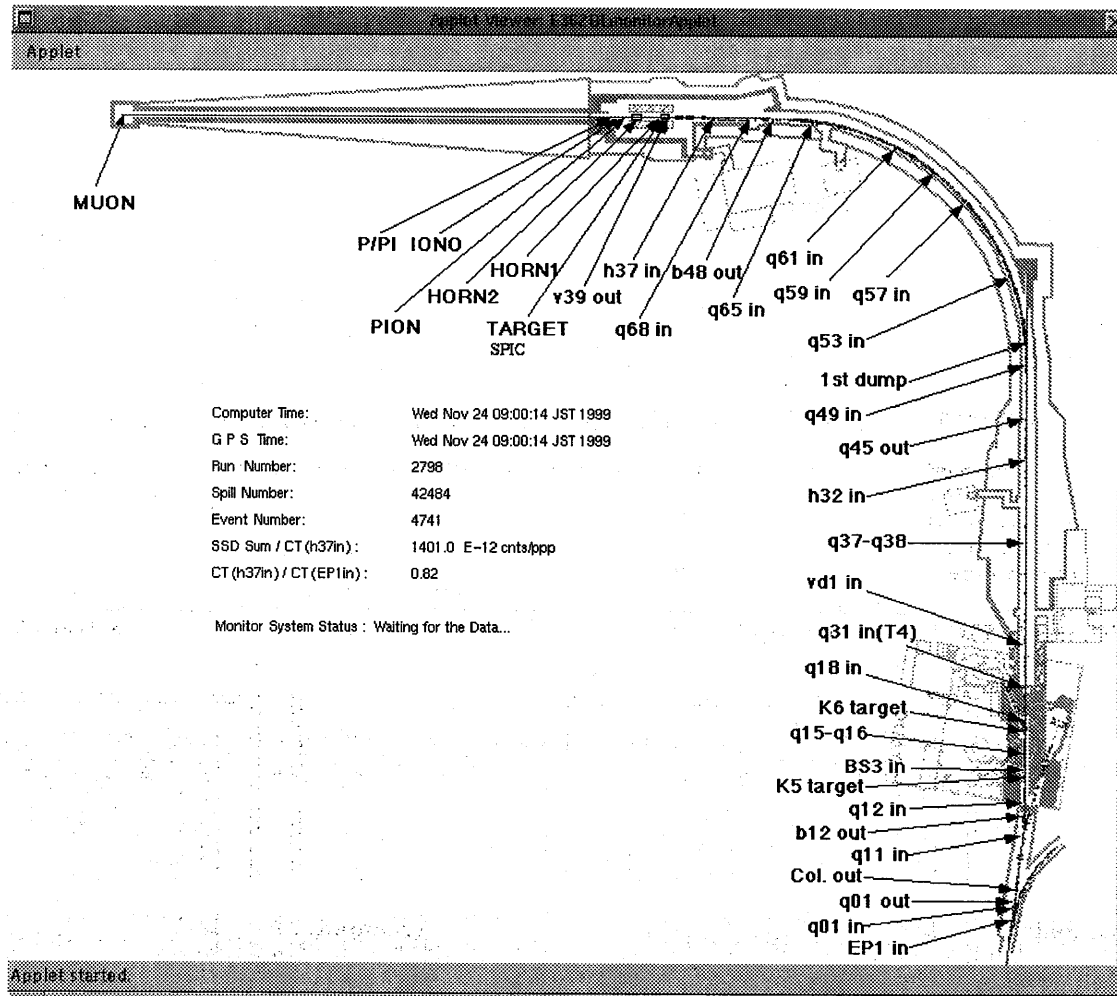
Figure 2.13: Monitors in the neutrino beam-line
