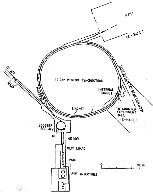
Figure 2.1: Schematic view of the 12GeV Proton Synchrotron
