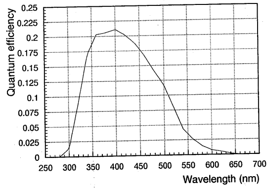
Figure 2.21: Quantum efficiency of 20-inch PMT as a function of wavelength of photons
