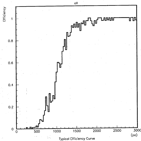
Figure 5.1: Typical threshold curve of FADC cut as a function of number of collected photoelectrons by inner PMTs.
