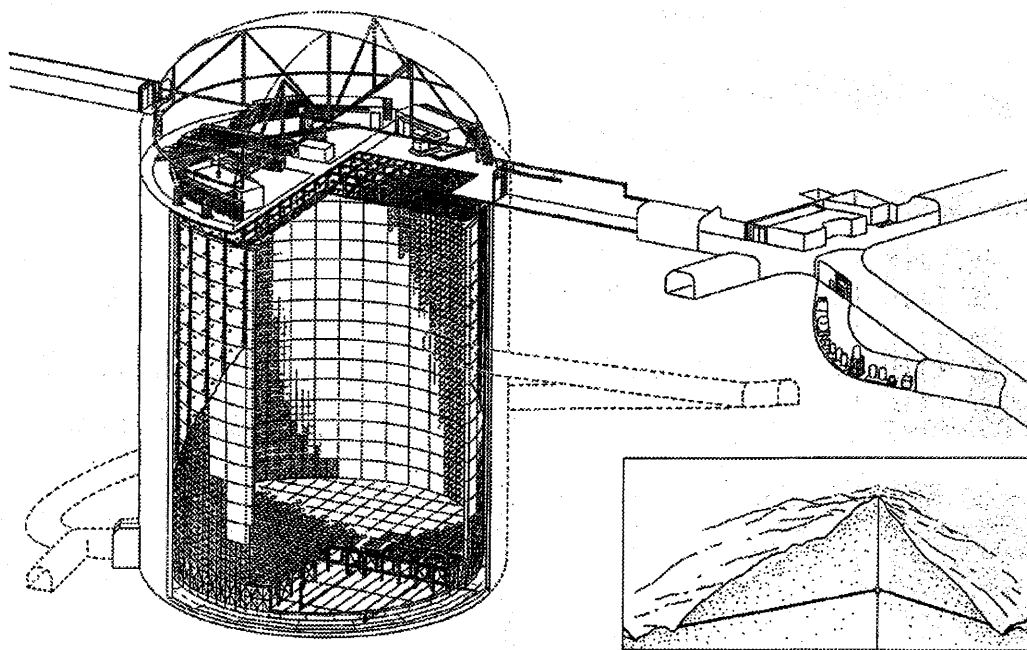
Figure 2.18: Schematic view of the Super-Kamiokande detector
