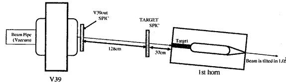
Figure 2.4: A schematic view of the SPICs, between the last magnet and the target
