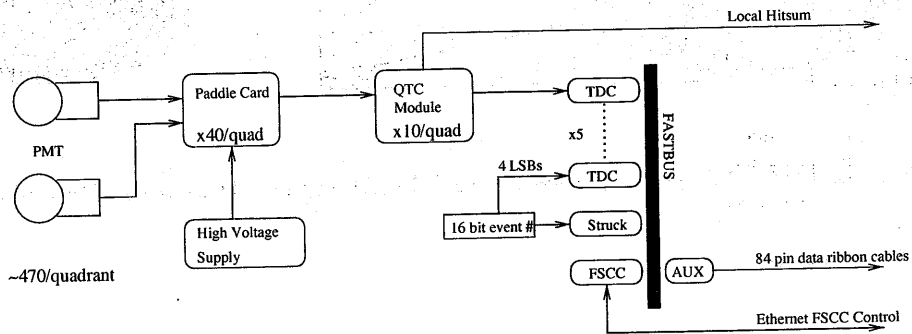
Figure 2.24: Outer detector acquisition system
