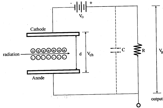
Figure 2.11: The principle of the ionization chamber
