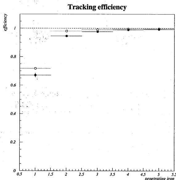
Figure 2.41: Tracking efficiency of the muon range chamber (MUC), as a function of number of iron plates transversed, where filled (open) circles are cosmic-ray data (our MC simulation).
