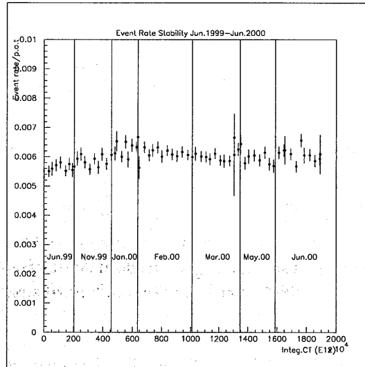
Figure 5.5: Long-term stability of the neutrino event rate observed at KT. Each point represents an event rate averaged over 2 days with a statistical error bar. In June '99, the neutrino beam intensity is lower than the other months due to the lower current in the horn magnet. In November '99, the detector configuration was slightly changed from the other period and the event rate looks slightly lower.
