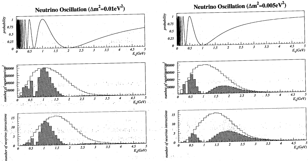
Figure 1.5: Neutrino energy spectrum distortion in the K2K in two \Delta m^2 cases ( \Delta m^2=0.01 (Left) and \Delta m^2=0.005 (Right), \sin^2 2\theta=1 ).
