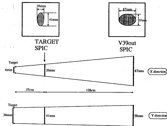
Figure 3.2: The schematic view of the proton beam emittance calculation. The shaded regions correspond to the 3\sigma contour given by a fit to the profile data assuming an Gaussian distribution.
