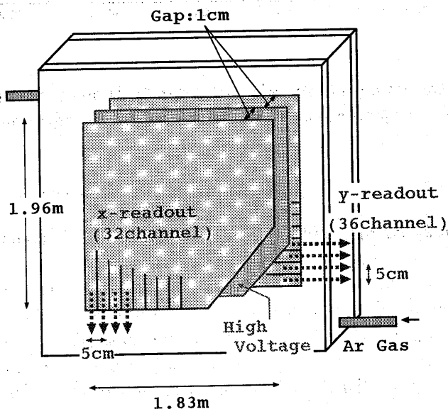
Figure 2.16: Schematic view of the muon monitor.
