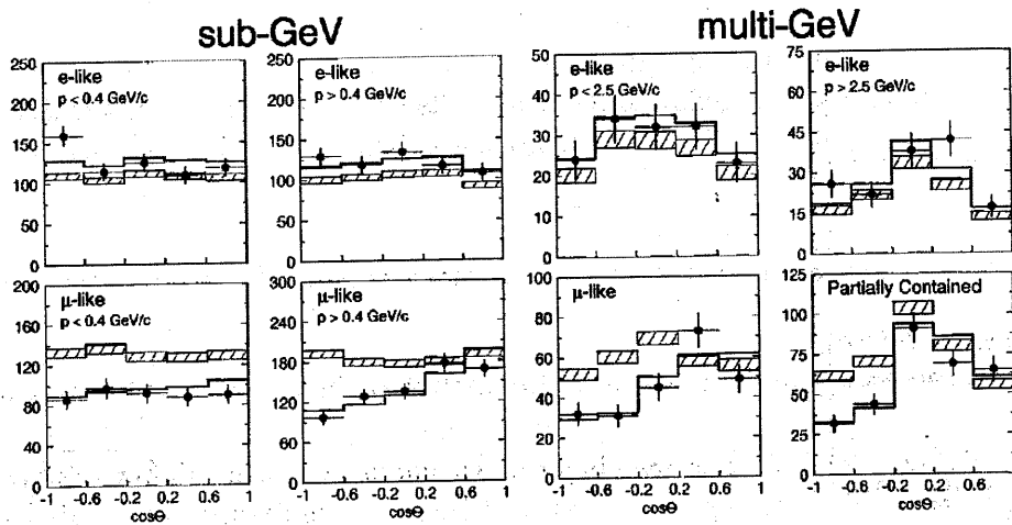
Figure 1.1: Zenith angle distribution of \mu -like and e-like events for sub-GeV and multi-GeV data sets[24]. Upward-going particles have \cos\Theta \leq 0 and downward-going particles have \cos\Theta \geq 0 . Sub-GeV data are shown separately for p \leq 400 \text{ MeV/c} and p \geq 400 \text{ MeV/c} . Multi-GeV e-like distributions are shown for p \leq 2.5 \text{ GeV/c} and p \geq 2.5 \text{ GeV/c} and the multi-GeV \mu -like are shown separately for FC(Fully Contained in the Super-Kamiokande detector) and PC(Partially contained in the Super-Kamiokande detector) events. The hatched region shows the Monte Carlo expectation for no oscillations. The bold line is the best fit for \nu_\mu \leftrightarrow \nu_\tau oscillations with the overall flux normalization fitted as a free parameter.
