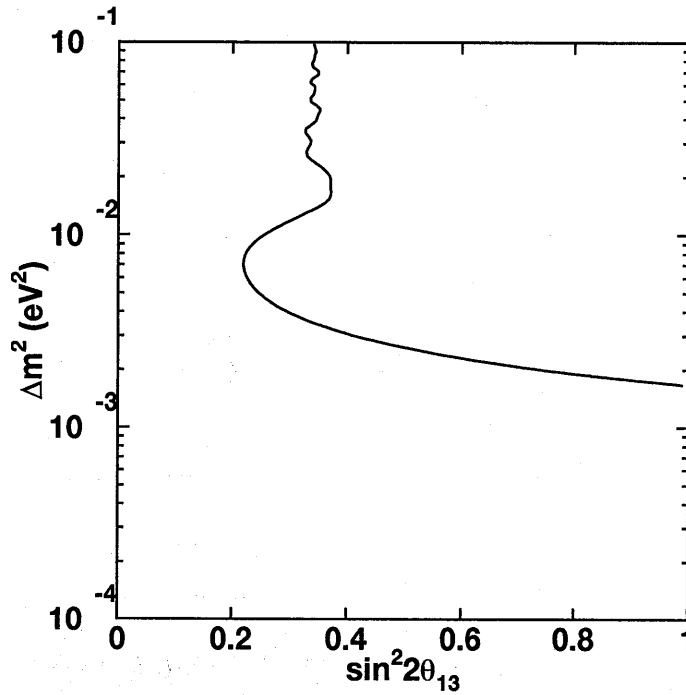
Figure 8.2: The 90% C.L. designed sensitivity of this experiment ( 10^{20} POT in 4 years) for \nu_\mu \rightarrow \nu_e oscillations assuming one mass scale dominance and \sin^2 2\theta_{23} = 1 . The excluded region of \sin^2 2\theta_{13} and \Delta m^2 is to the right side to the curve.
