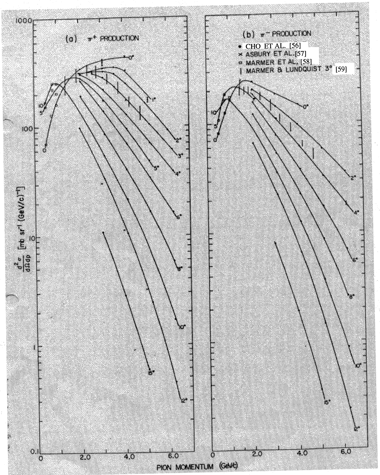
Figure 3.5: Results of the pion production measurements[72, 73, 74, 75] and fitted results by Sanford-Wang formula[67]. Left figure: \pi^+ , right figure: \pi^- .
