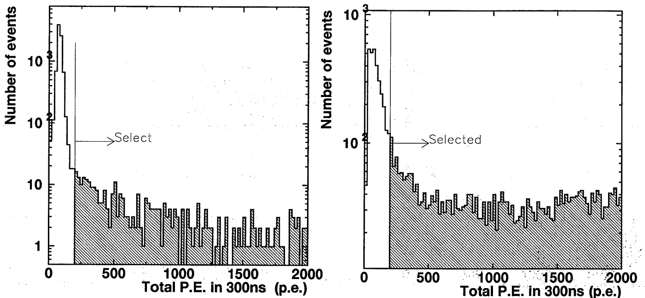
Figure 6.1: Number of total photo-electrons in 300ns time window in SK for data (left figure) and for MC (right figure) after the decay electron cut. Most of unselected events in the MC sample are generated by NC interactions, while these in data are from the low-energy events like gamma rays from the rock.
