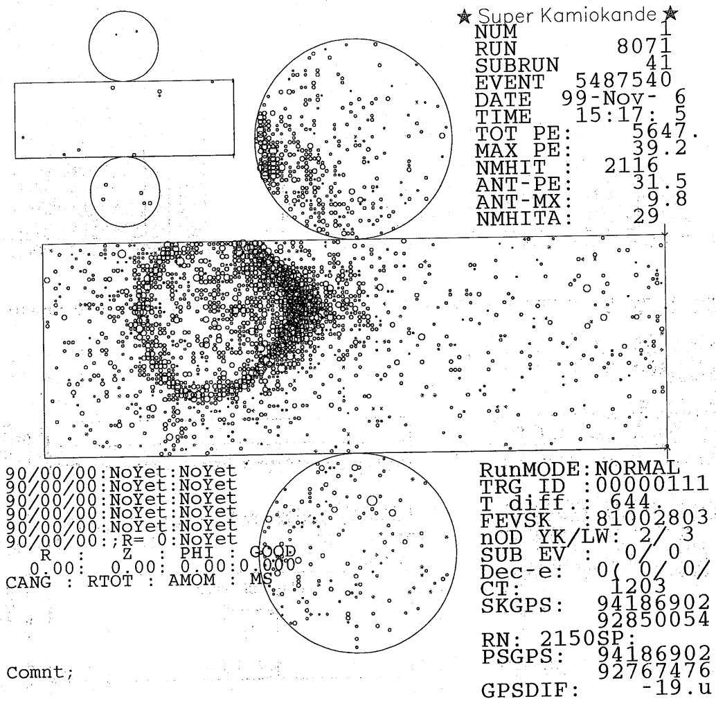
Figure 6.9: The event display of the singl-ring e-like FC event observed in Super-Kamiokande. The deposit energy is 594MeV/c. It points back to the KEK-PS \nu beam with an angular deflection of 16.4 degrees.
