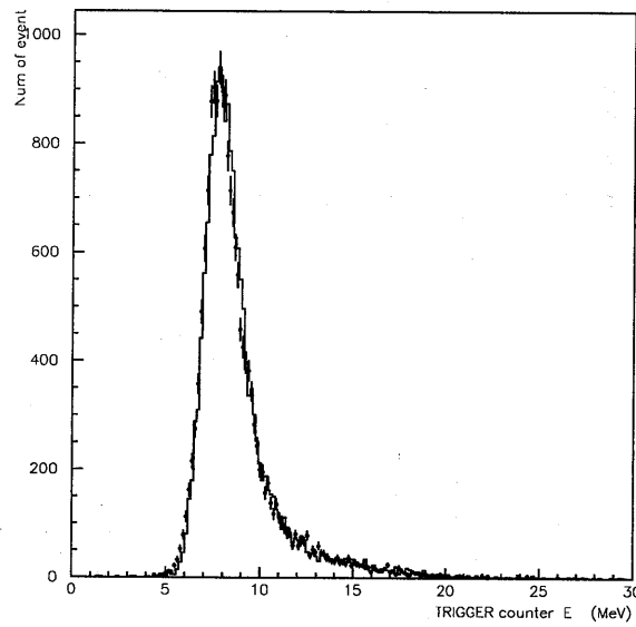
Figure 2.31: Trigger counter energy distribution measured in a cosmic ray test. The points with error bars represents data, while solid histograms are from a simulation.
