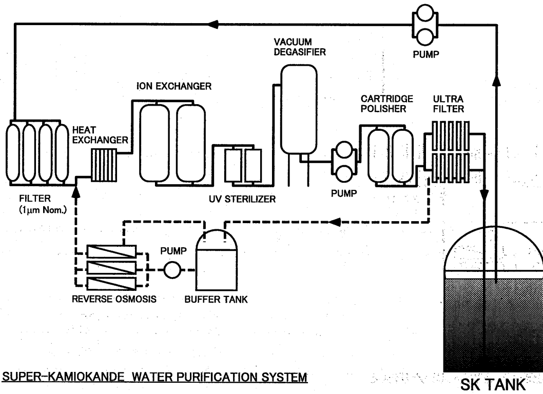
Figure 2.25: Water purification system.
