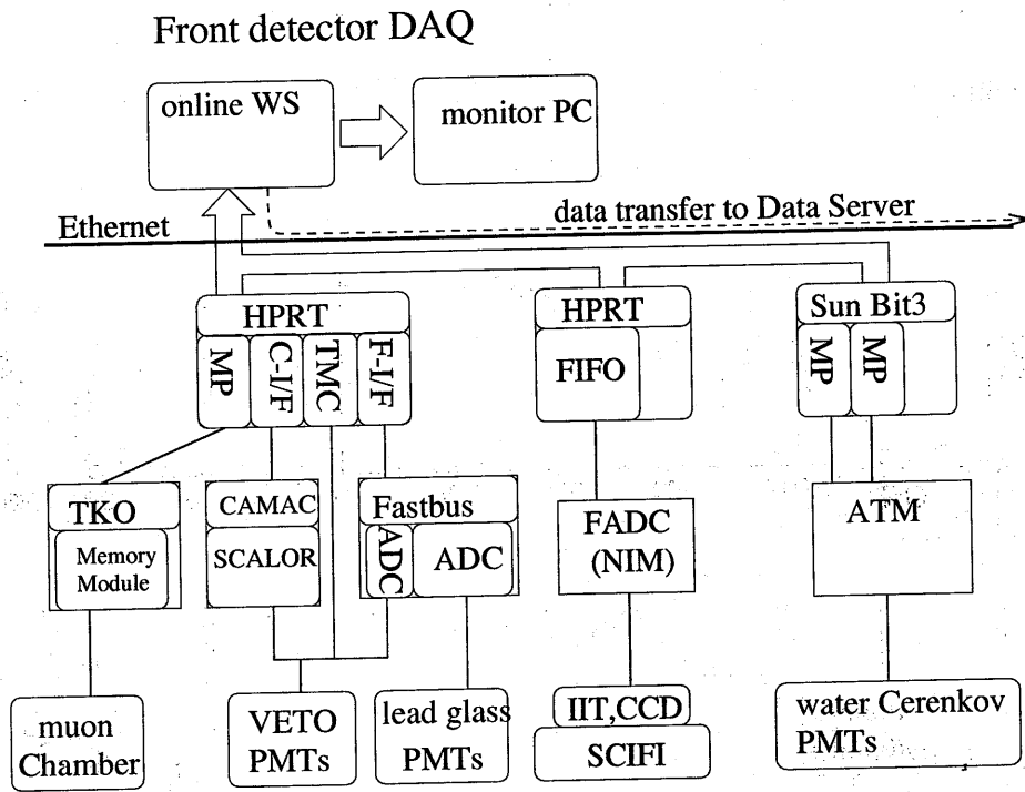
Figure 2.43: Near detector data acquisition system
