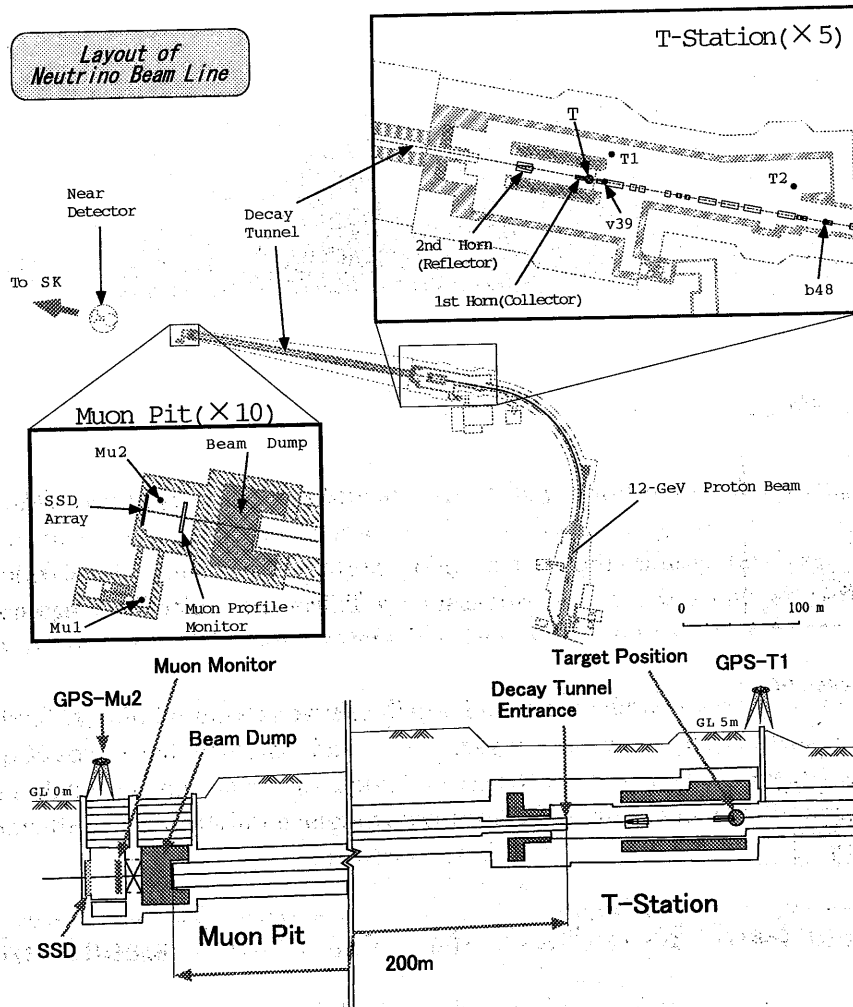
Figure 2.3: Schematic view of the neutrino beam-line and near detector, after 12GeV-PS
