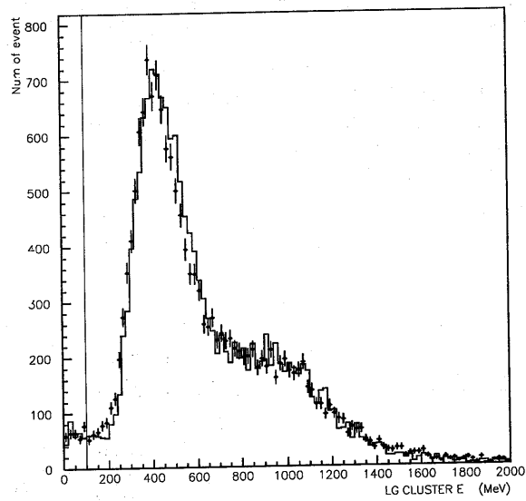
Figure 2.39: LG cluster energy distribution for cosmic-ray muons. Filled circles with error bars are the data, and solid histograms are our MC simulation.
