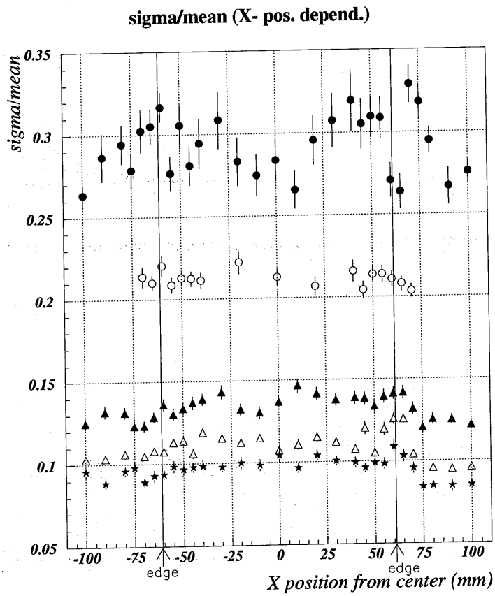
Figure 2.37: Dependence of energy resolution on incident position for electron beam. Electrons of different incident energies were measured. The black circles are 100\text{MeV} , white circles are 200\text{MeV} , black triangles are 500\text{MeV} , white triangles are 800\text{MeV} , and stars are 1000\text{MeV} .
