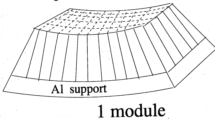
Figure 2.34: One module of the Lead Glass Calorimeter
