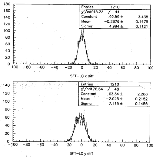
Figure 2.32: Trigger counter position residual distribution. The Upper figure is the horizontal direction, the lower one is the vertical direction.
