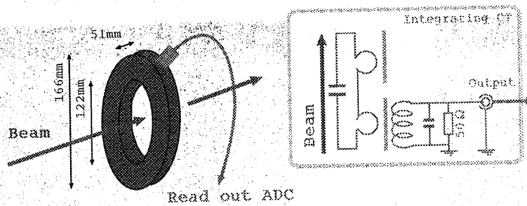
Figure 2.9: Schematic view of the CT
