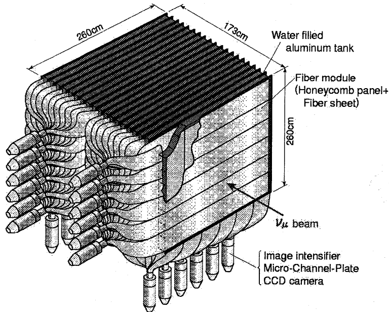
Figure 2.29: Schematic view of the scintillation fiber tracker with the water target.
