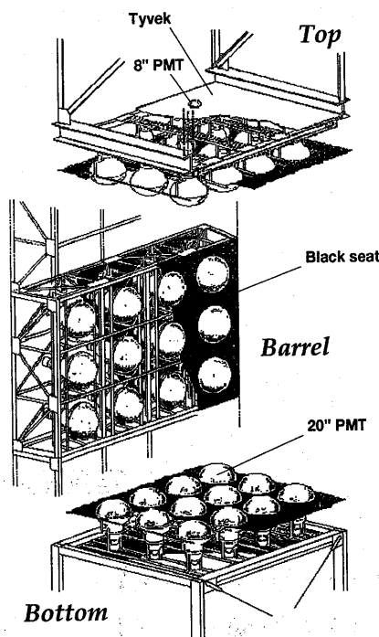
Figure 2.19: Schematic view of the frame which supports PMTs.
