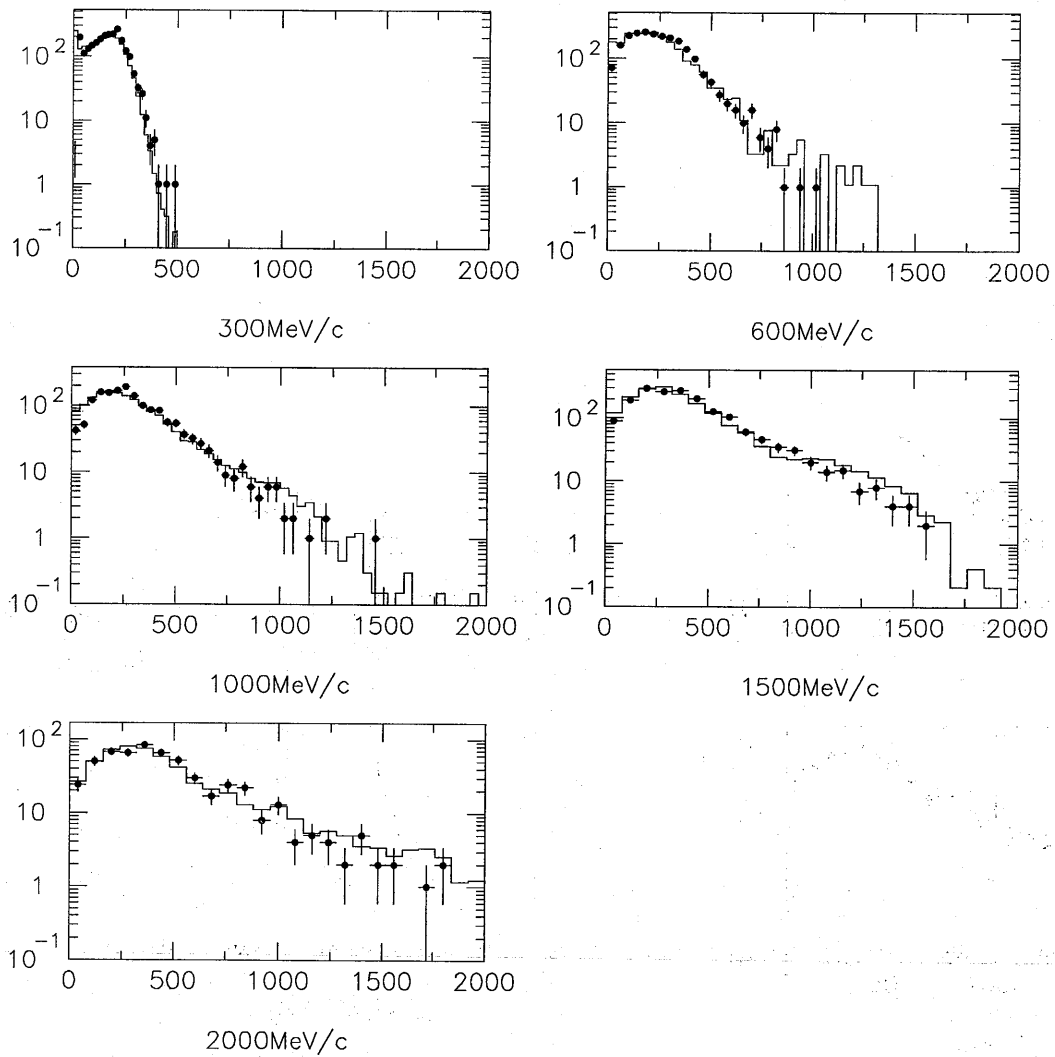
Figure 2.38: Responses for charged pions at different beam momenta. The filled circle with an error bar are data, the solid histograms are our MC simulation.
