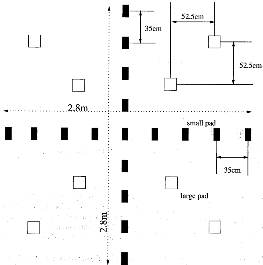
Figure 2.17: Configuration of the silicon pad detectors.
