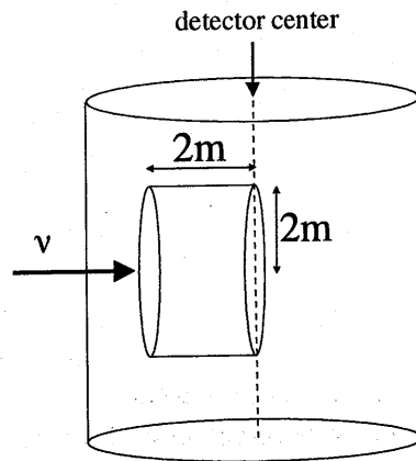
Figure 5.3: The definition of fiducial volume in KT
