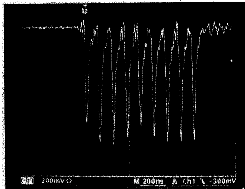
Figure 2.2: Oscilloscope picture of the micro-structure in the beam
