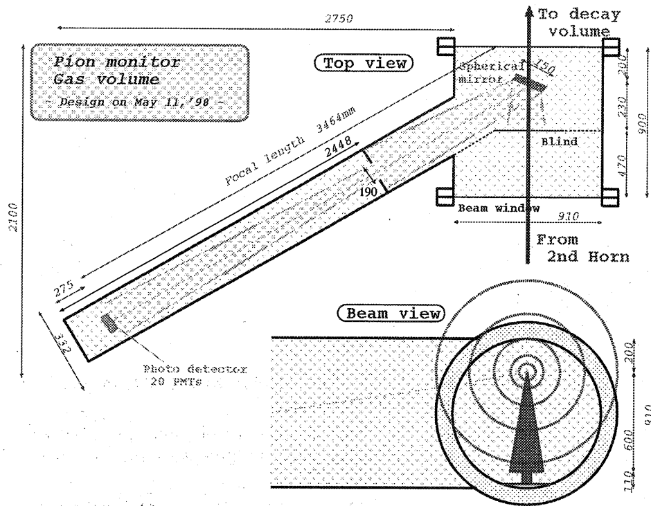
Figure 2.14: Schematic view of the pion monitor (PIMON).
