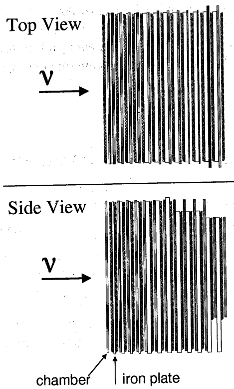
Figure 2.40: Schematic view of muon range detector.
