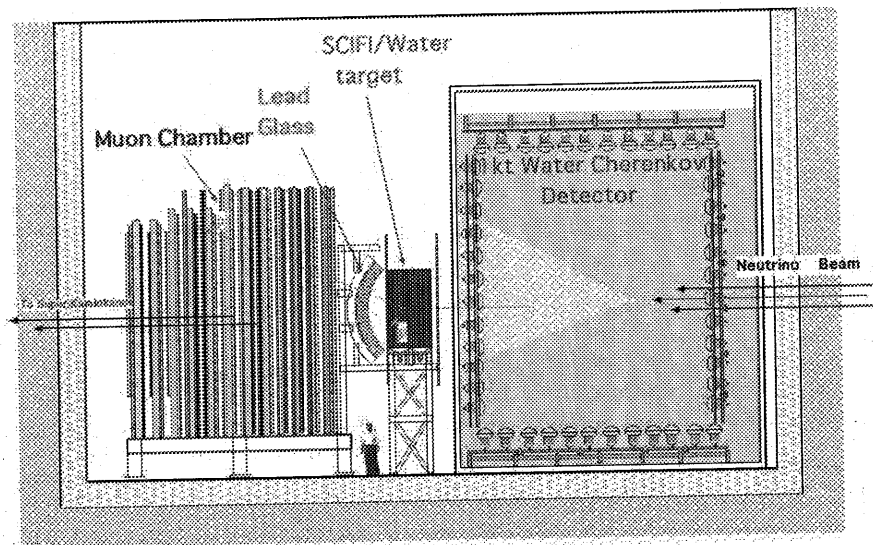
Figure 2.26: Schematic view of the near detectors
