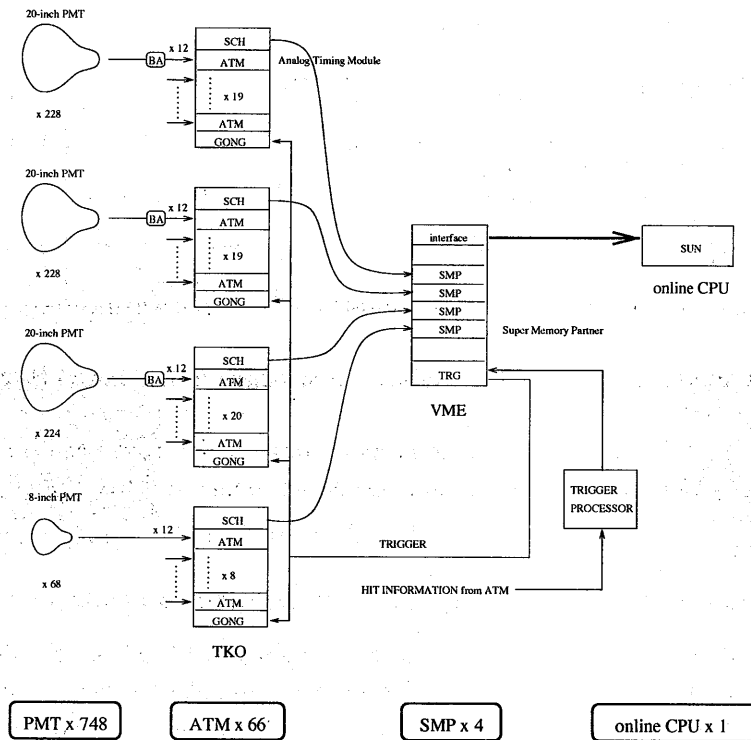
Figure 2.27: Data acquisition system for the 1kt water Cherenkov detector (KT)
