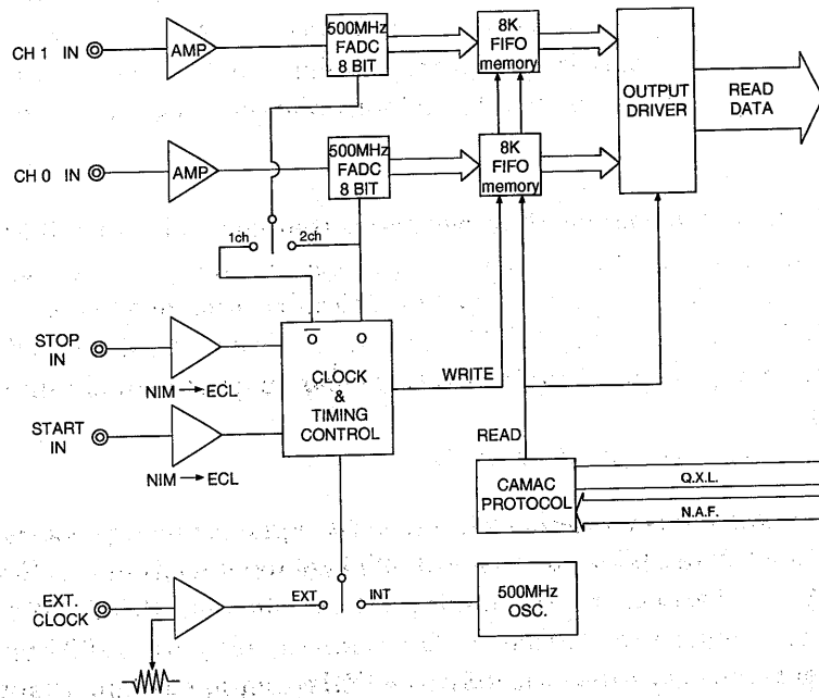
Figure 2.28: Block diagrams of the transient digitizer used in KT
