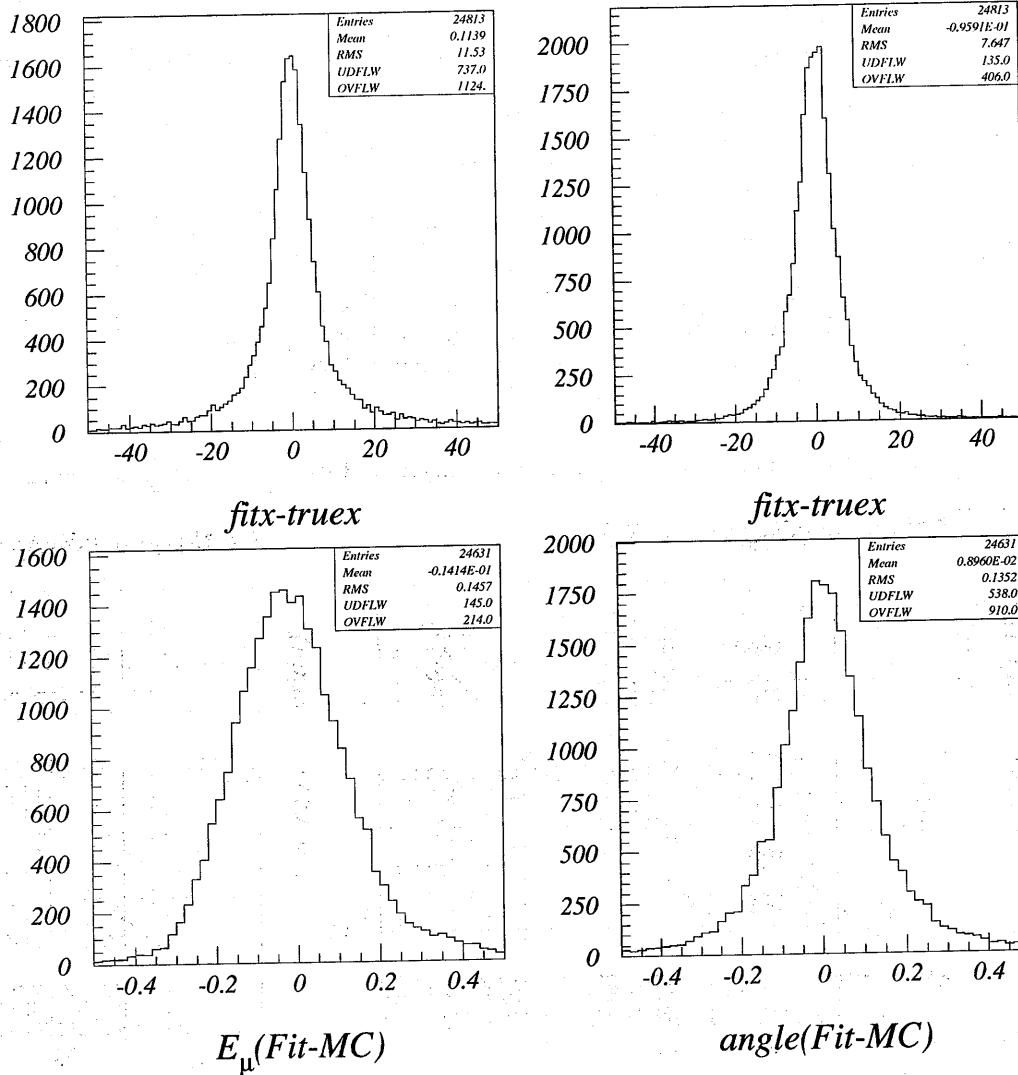
Figure 2.42: Tracking residual distribution of muon range chamber (MUC). The upper left figure is the position distribution in the horizontal direction, the upper right figure is the position distribution in the vertical direction, the lower left figure is the energy distribution and the lower right figure is the angular distribution.
