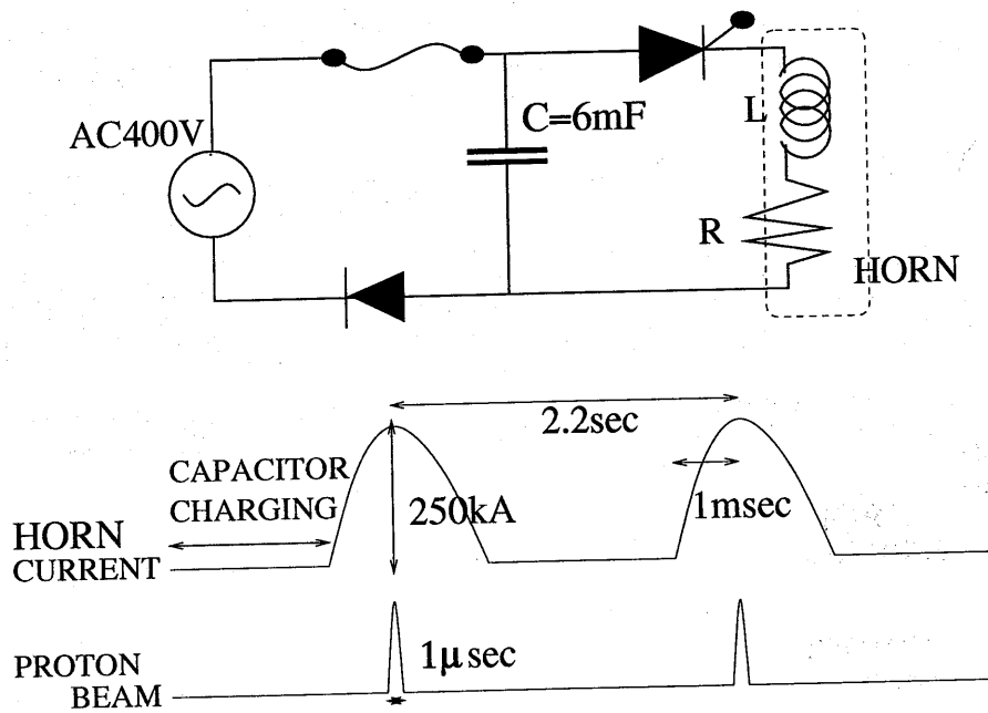
Figure 2.6: The pulsed current supplied to horn magnets[48]
