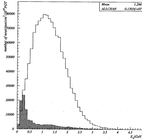
Figure 2.7: Performance of our horn system. The shaded (solid) histograms show the MC simulated neutrino flux at SK with the current supplied to the horn magnets of 0kA (250kA), where the target diameter is target is 30mm \phi
