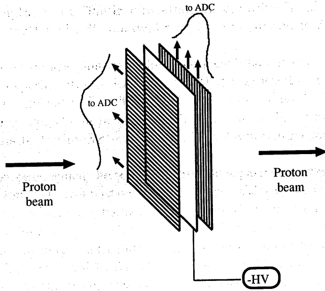
Figure 2.12: Schematic view of the SPIC used in K2K.
