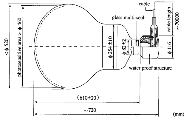
Figure 2.20: Schematic view of 20-inch PMT used in the inner detector (Hamamatsu R3600).
