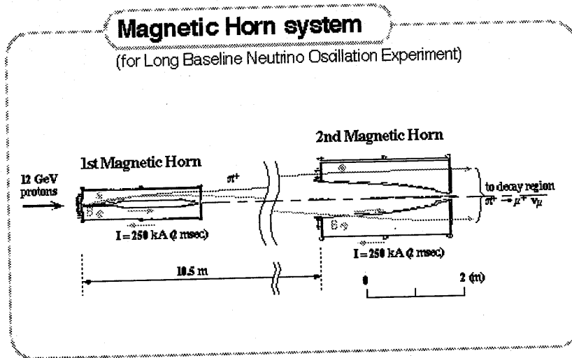
Figure 2.5: Schematic view of the horns.
