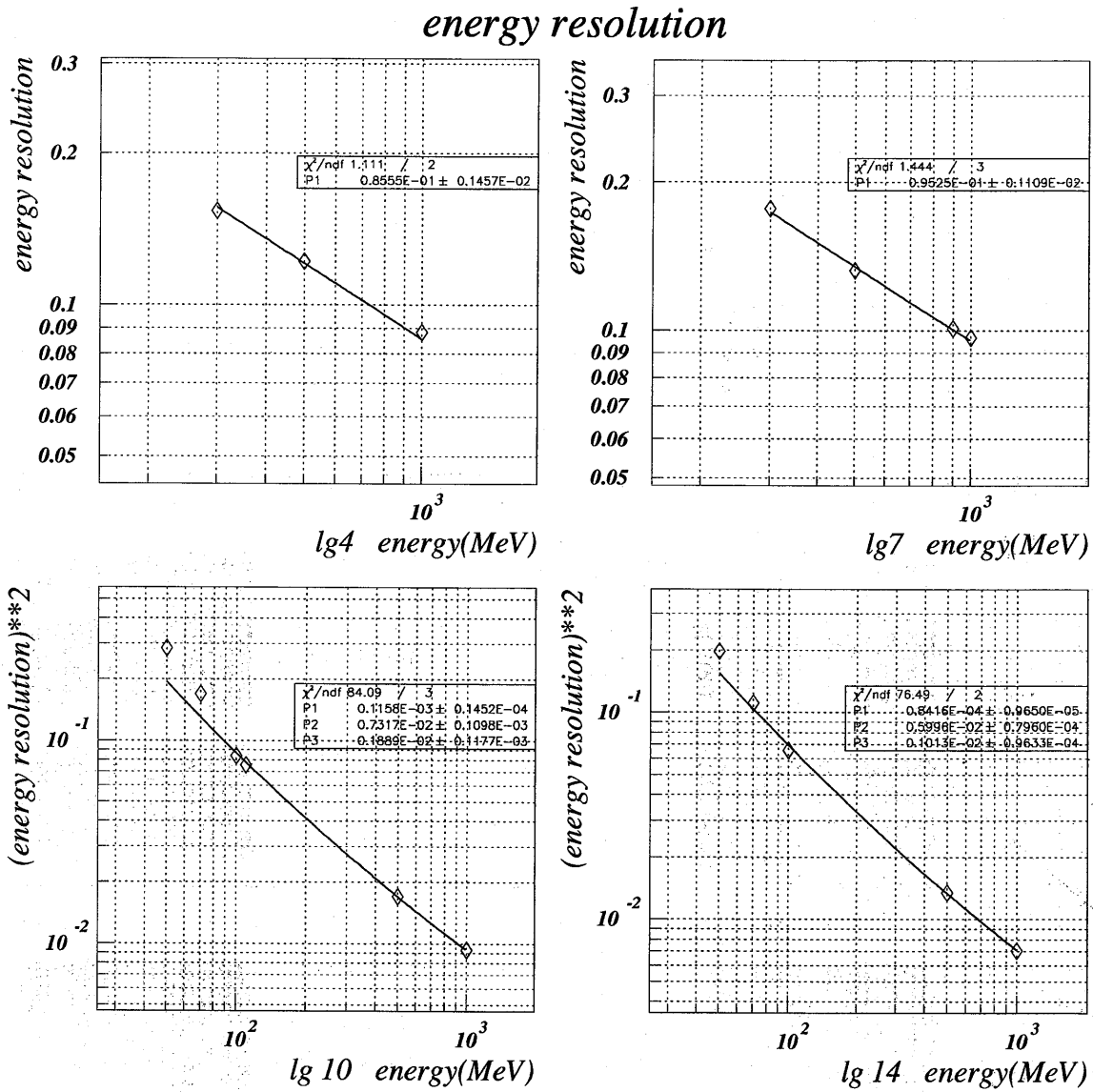
Figure 2.36: Energy resolution for electron beam. On the horizontal axis are incident energies and on the vertical axis are energy resolutions. The lines are fitting results. The upper figures use only \sigma_1 for fitting. As low energy region measurements had been conducted, the lower figures use the function (\frac{\sigma(E)}{E})^2 = \frac{\sigma_0^2}{E^2} + \frac{\sigma_1^2}{E} + \sigma_2^2 for fitting.
