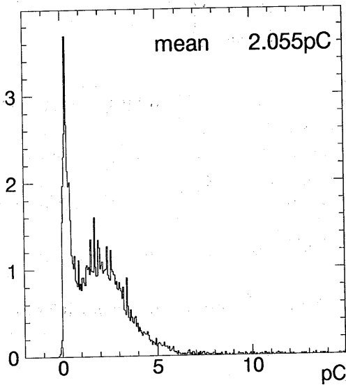
Figure 2.22: One photoelectron distribution measured by 20-inch PMT
