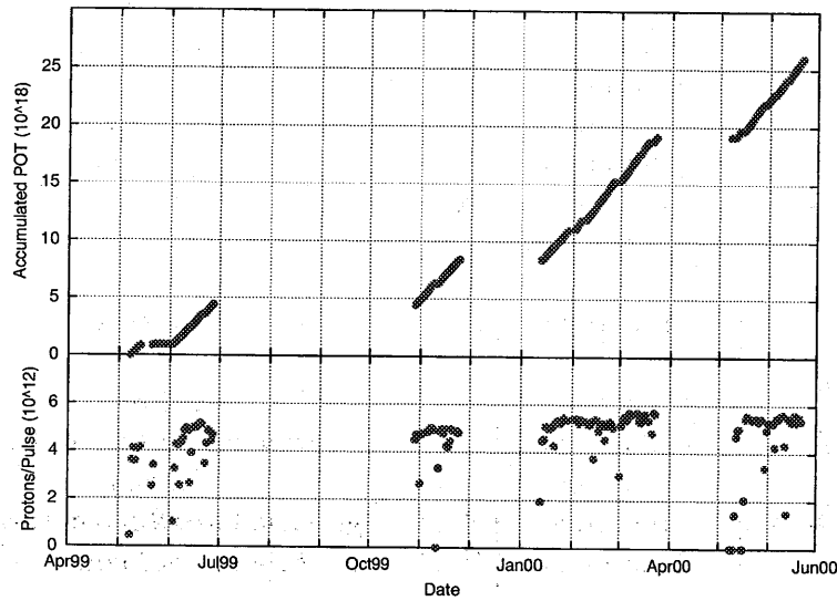
Figure 2.10: (Upper) Integrated number of protons on the target since May 1999 till June 2000. (Lower) Intensity of the proton beam at the target in the unit of protons per pulse (ppp).
