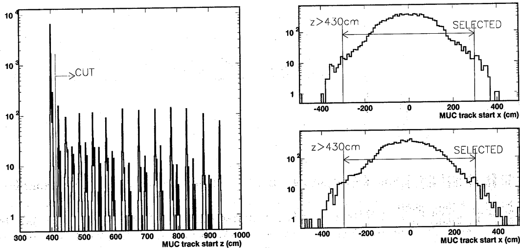
Figure 4.5: MUC track start position distribution. The left figure shows the distribution along the beam axis ( z -position), and the upper (lower) right figure is a projection on to the horizontal (vertical) axis after the z -position cut. The neutrino interactions in the iron plate and incoming cosmic-ray muons are rejected by the z -position cut and the horizontal (vertical) position cut, respectively.
