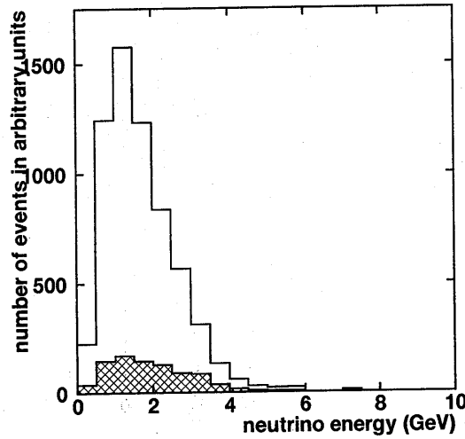
Figure 7.3: The kaon contribution in the selected MC events induced by \nu_e as a function of \nu_e energy. Blank histogram corresponds to the selected MC events induced by \nu_e from pion decays and shaded histogram corresponds to that from kaon decays.
