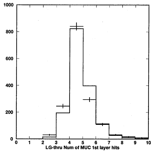
Figure 4.9: The number of hit cells in the MUC first layer distribution. The histograms correspond to the \nu_\mu MC normalized to the data by entries.
