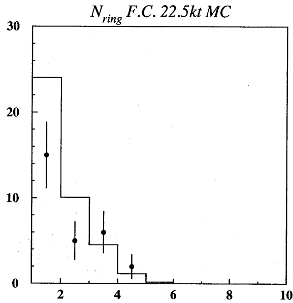
Figure 6.6: Number of Cherenkov rings distribution of the selected beam-induced FC events for data (filled circles with an error bar) and for MC (solid histograms).
