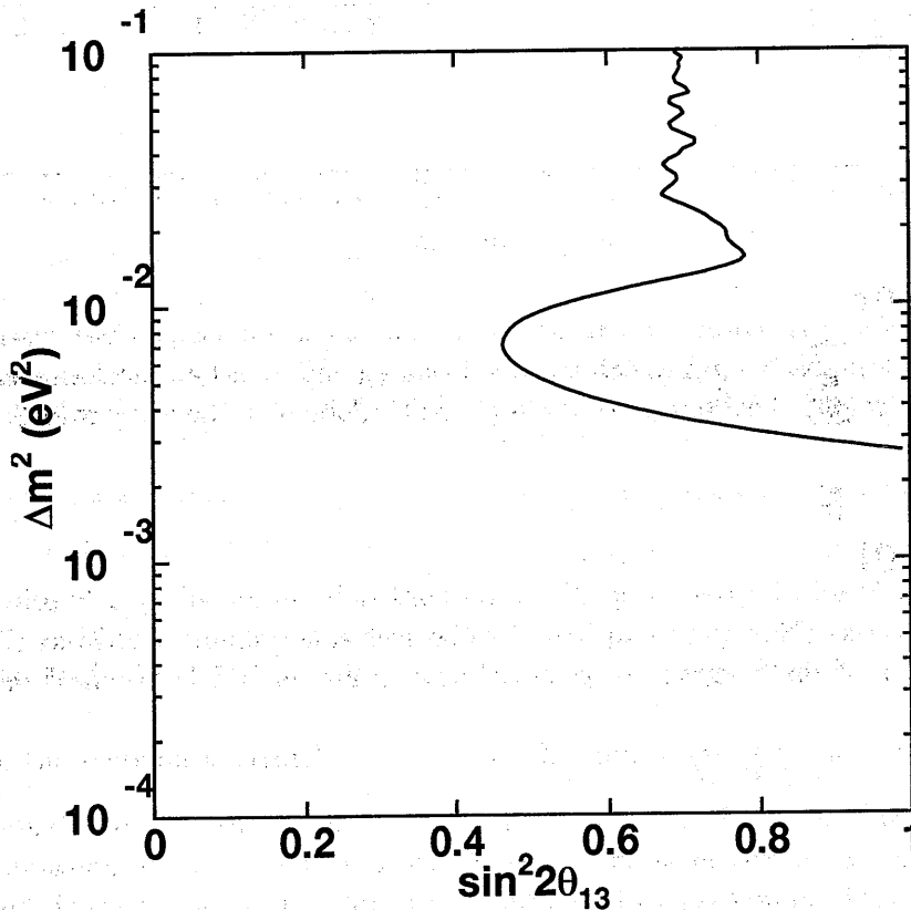
Figure 8.1: The 90% C.L. upper limit on \nu_\mu \rightarrow \nu_e oscillations assuming one mass scale dominance and \sin^2 2\theta_{23} = 1 . The excluded is the area to the right side of the curve.
