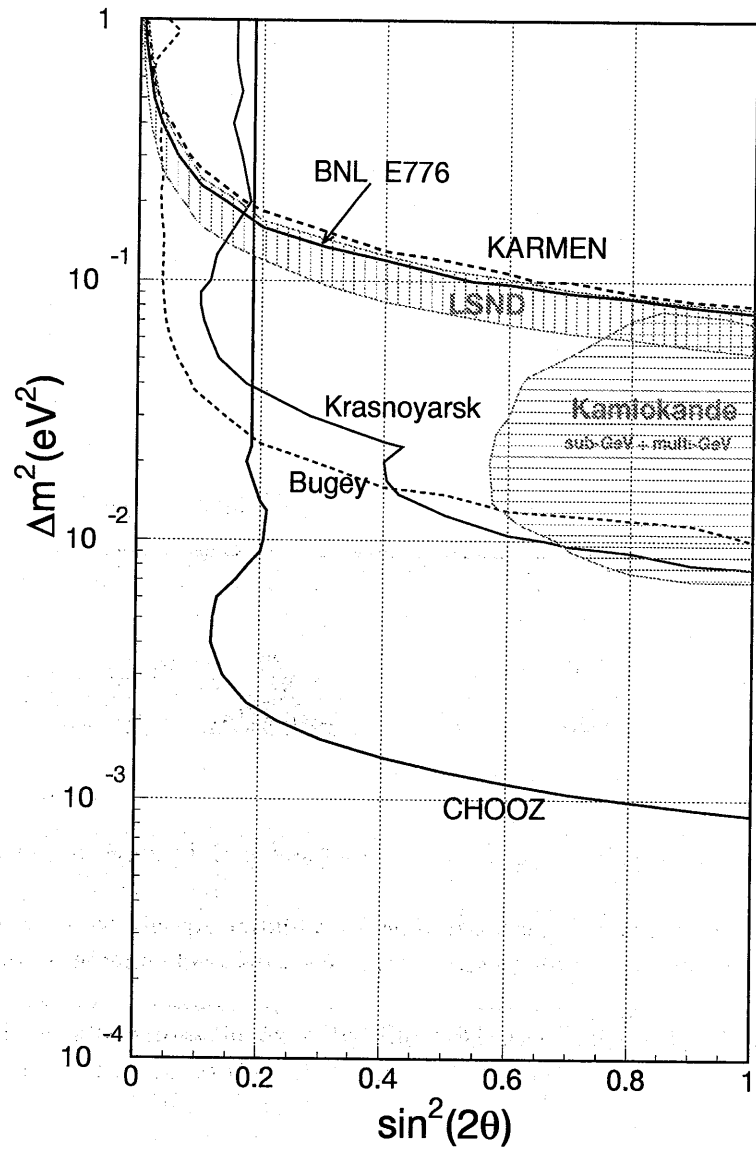
Figure 1.2: Allowed (shaded areas) and excluded (lines) regions of parameter space for \nu_\mu \rightarrow \nu_e or \bar{\nu}_e \rightarrow \bar{\nu}_\mu oscillations. The excluded regions lie on the right side of curves.
