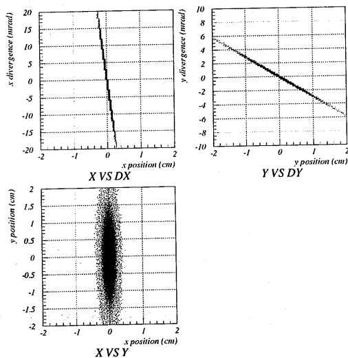
Figure 3.3: The results of the proton beam emittance calculation. Top-Left: x vs dx ( x is the horizontal position, dx is the horizontal divergence of the beam), Top-Right: y vs dy , Bottom-Left: x vs y (proton beam profile at the target)
