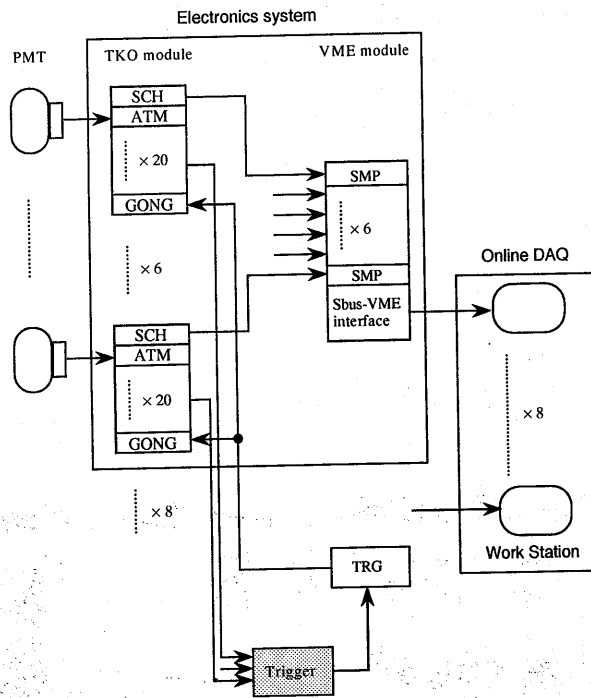
Figure 2.23: Inner detector data acquisition system
