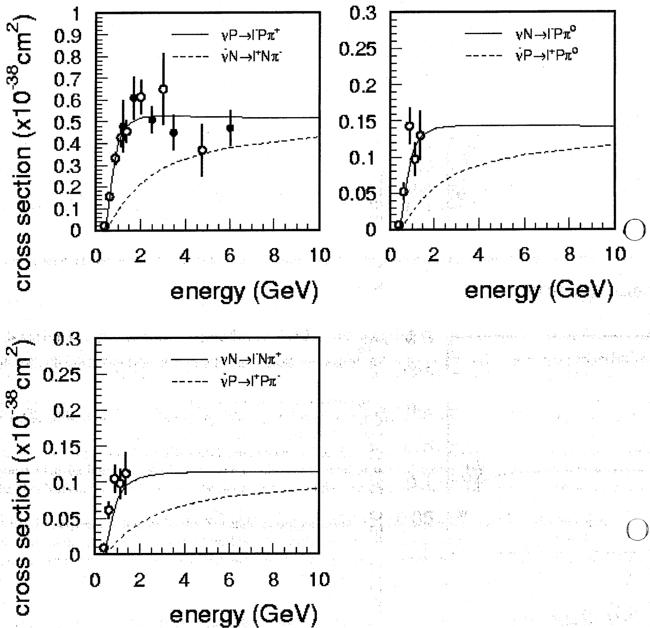
Figure 3.11: Calculated cross sections of the charged current single pion production reaction. Open circles with error bars show the result of the ANL experiment[81], and closed circles show that of the GGM experiment[82].
