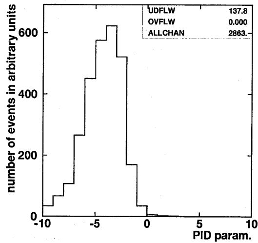
Figure 7.4: Particle ID parameter for fully-contained 1-ring MC events induced by the beam \nu_e CC quasi-elastic interactions. The negative (positive) value of the parameter corresponding to showering (non-showering) particle type. Misidentification probability is 0.5% for this sample.
