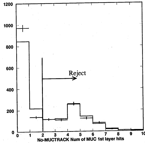
Figure 4.7: The number of hit cells in the MUC first layer distribution. The histogram corresponds to the \nu_\mu MC normalized to the data by entries.
