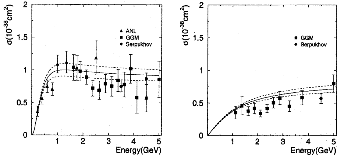
Figure 3.10: Calculated total cross sections of \nu_{\mu}n \rightarrow \mu^{-}p (left) and \bar{\nu}_{\mu}p \rightarrow \mu^{+}n (right) compared with the experimental data, ANL[81], GGM[82] and Serpukhov[83]. Upper and lower dashed lines show the cross section with M_A=1.11 and 0.91 , respectively.
