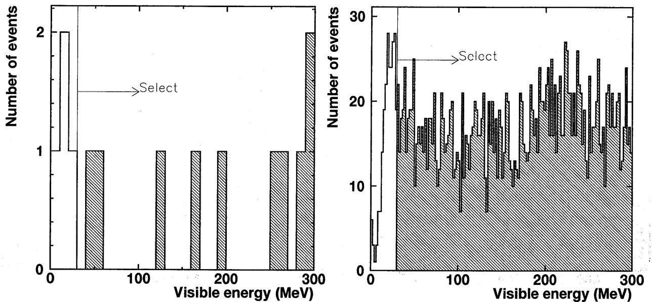
Figure 6.3: Reconstructed electron-equivalent energy distributions of SK FC events for data (left) and for MC (right) after the fiducial volume cut. Most of the unselected events in the MC sample are NC events.
