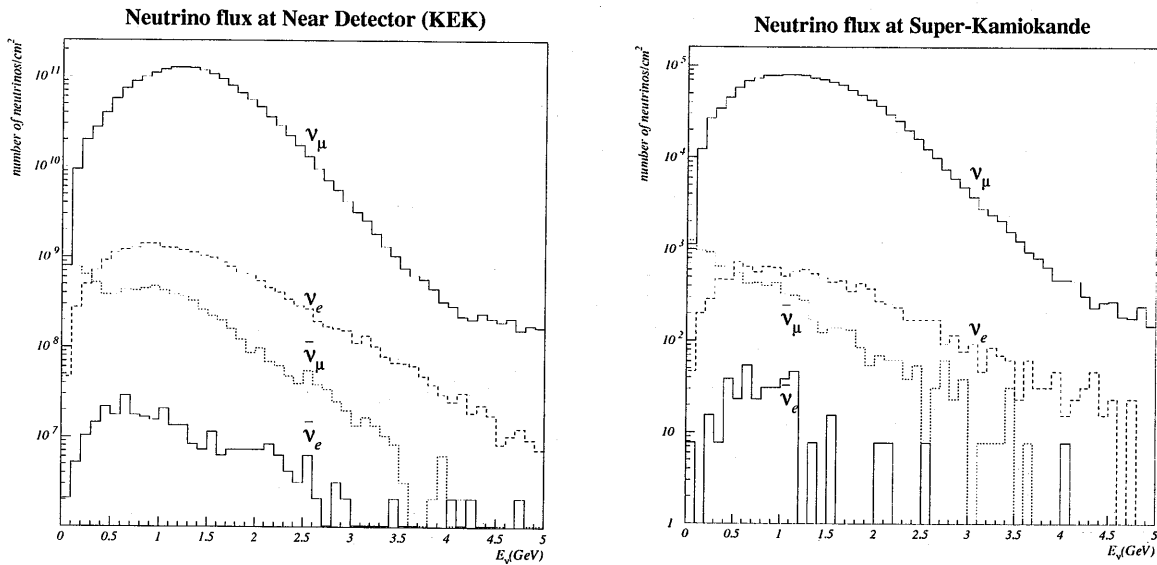
Figure 3.7: Neutrino flux calculation using the Monte Carlo simulation. (The Cho hadron production model is employed) Left figure: Neutrino flux at KEK, Right figure: Neutrino flux at SK
