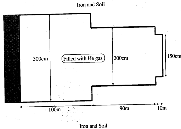
Figure 2.8: Schematic view of the decay pipe.
