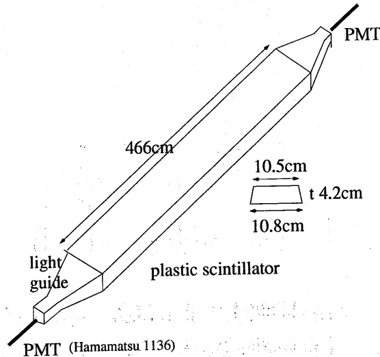
Figure 2.30: Schematic view of the trigger counter (TG).
