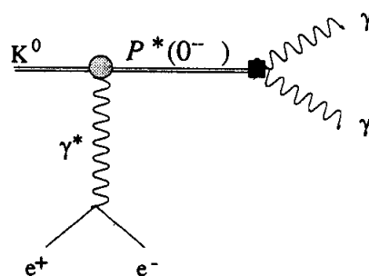
(b) Pseudoscalar state contribution
